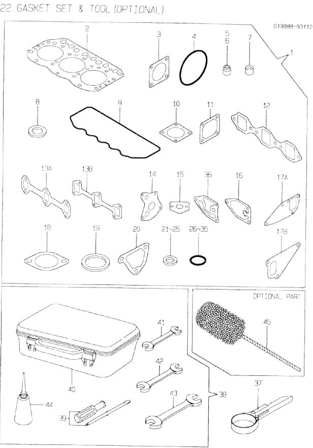
Fig.22. GASKET SET & TOOL(OPTIONAL)
