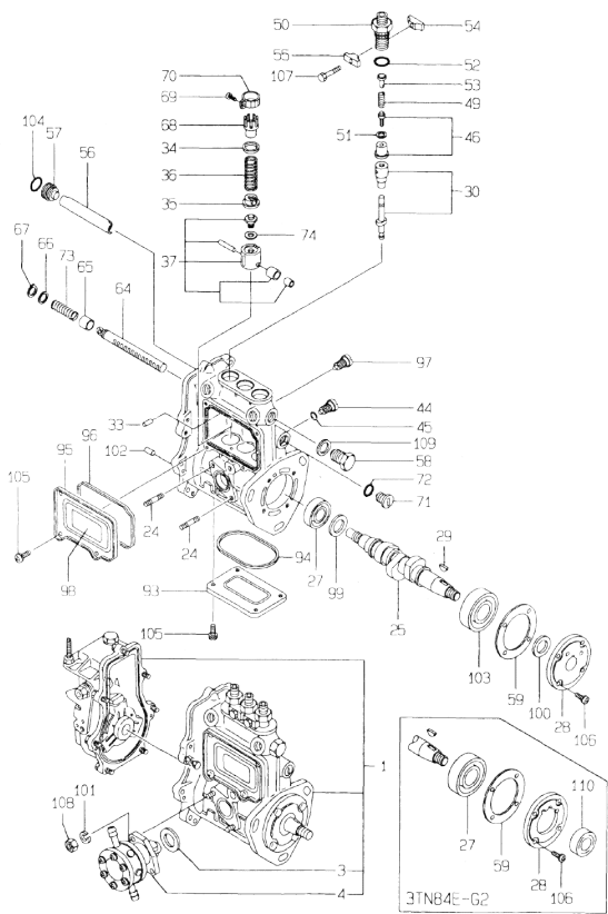
13.FUEL INJECTION PUMP
