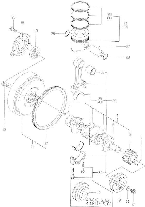
Fig.32. CRANKSHAFT & PISTON
