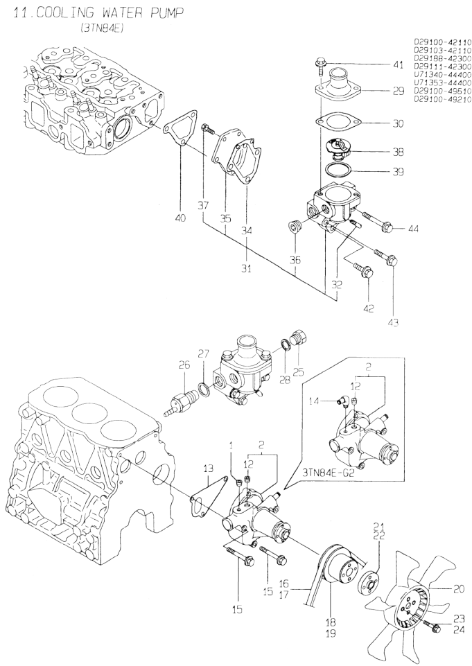
Fig.11. COOLING WATER PUMP(3TN84E)
