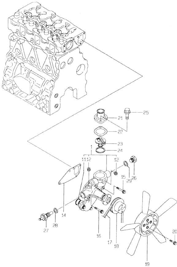
10.COOLING WATER PUMP (3TNC78E-S)
