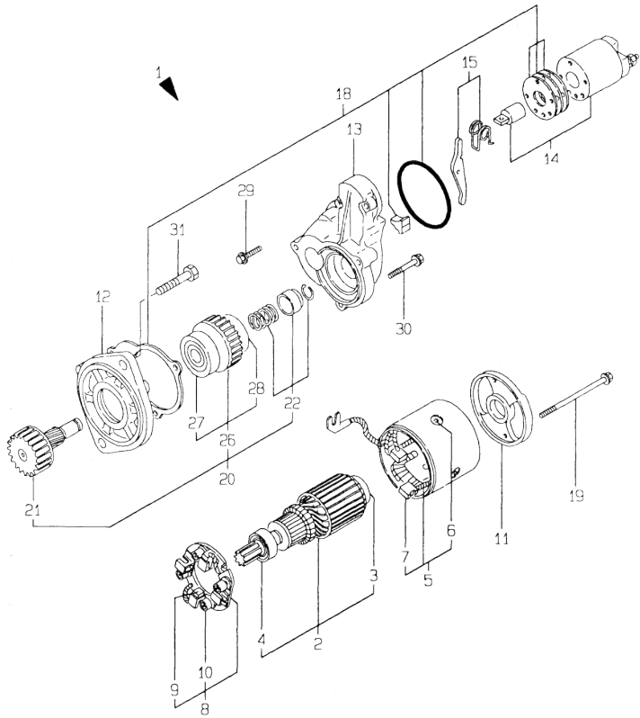
43.STARTING MOTOR (4TN84 (T) E-S, G2)
