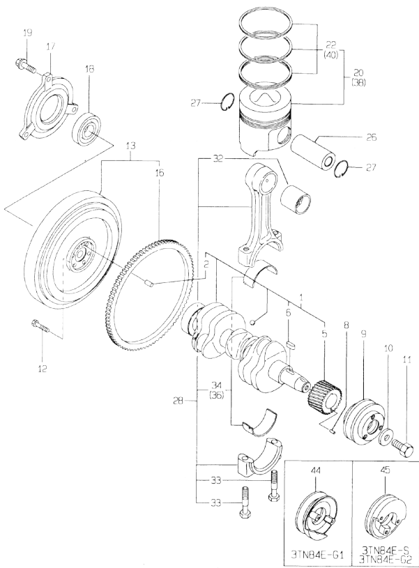
8. CRANKSHAFT & PISTON
