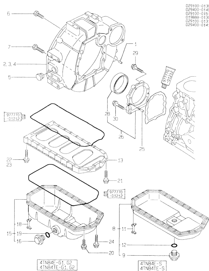
25. FLYWHEEL HOUSING & OIL SUMP
