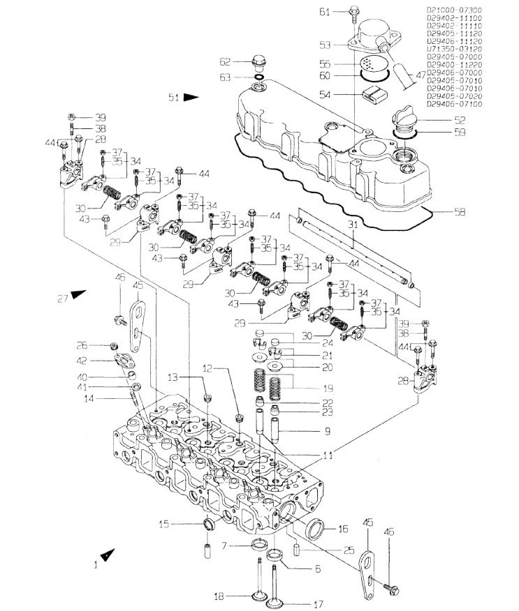
Fig.26. CYLINDER HEAD & BONNET
