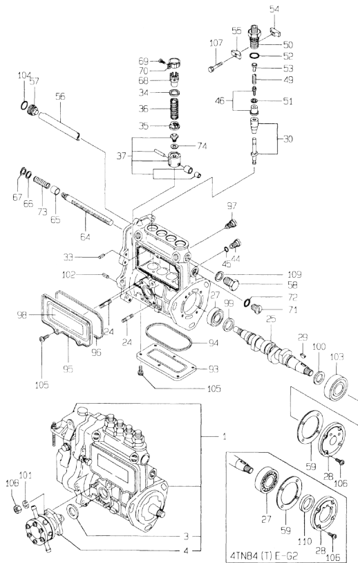
38.FUEL INJECTION PUMP
