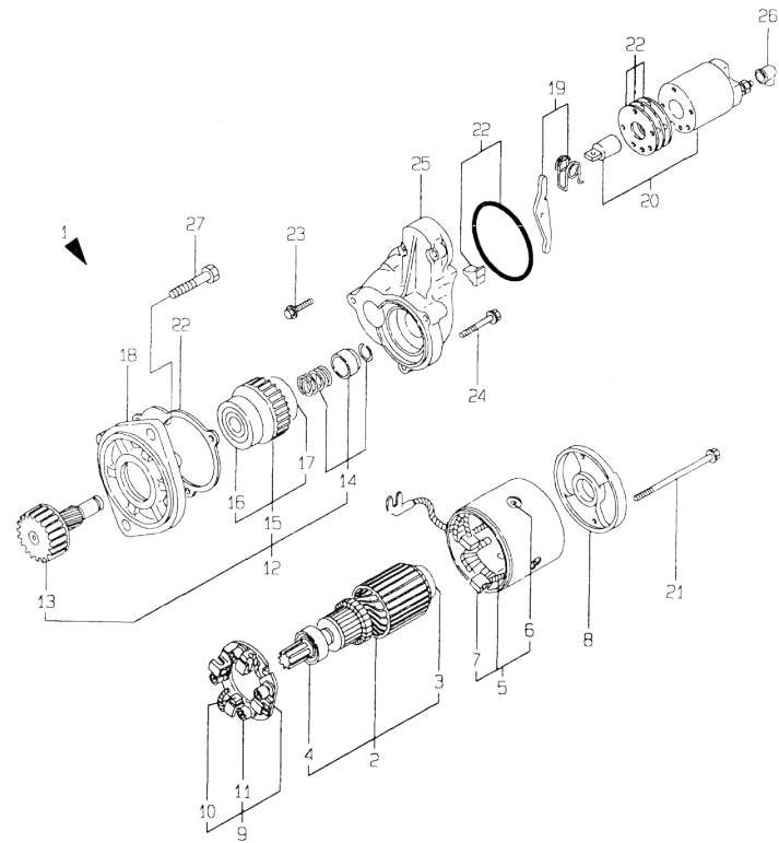
18. STARTING MOTOR
