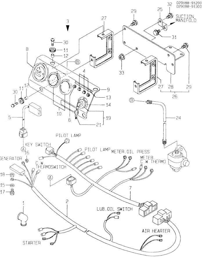
46 .PANEL
