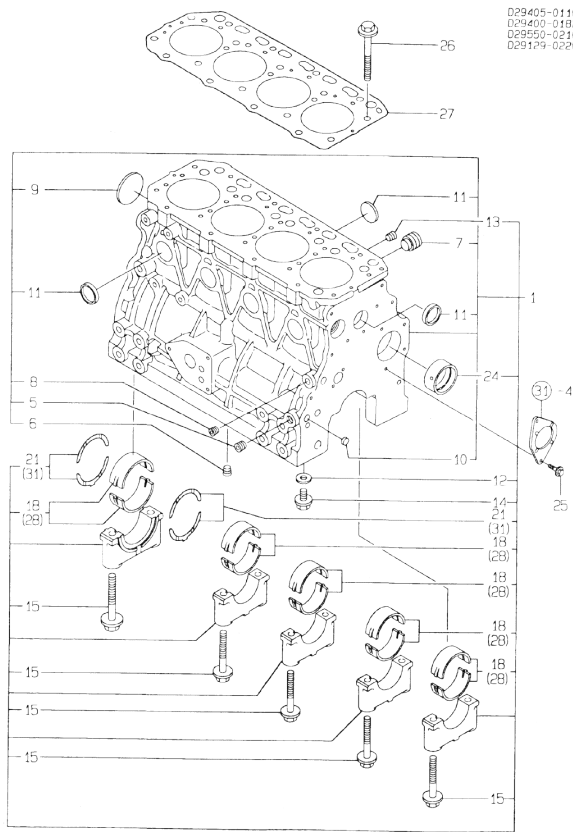
Fig.23. CYLINDER BLOCK
