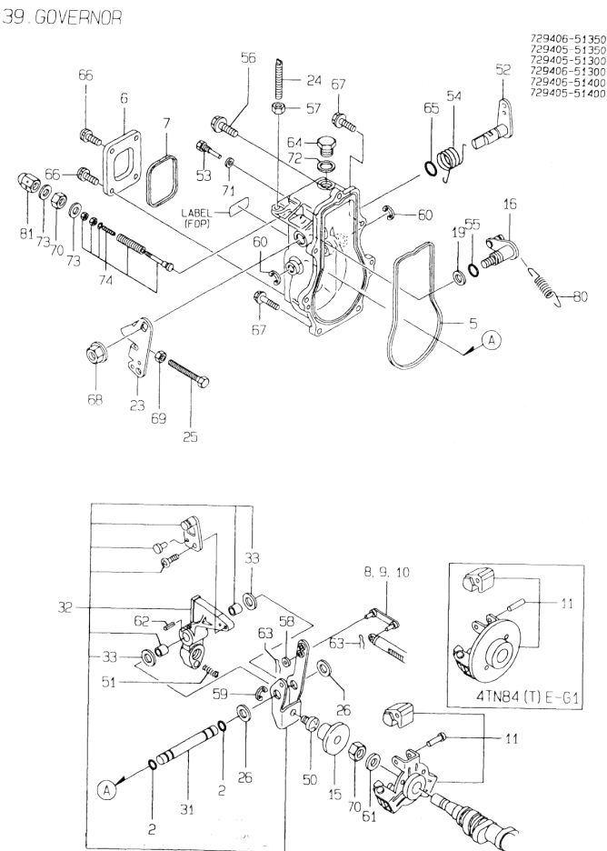
Fig.39. GOVERNOR
